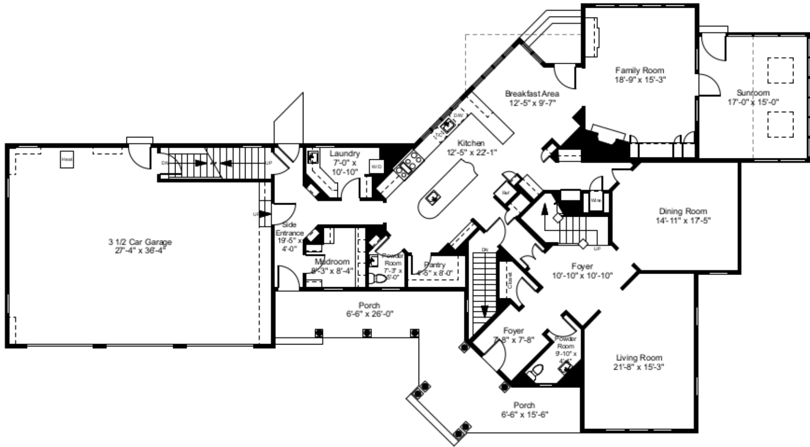
First Floor Plan Ceiling Height = 8'-8"
