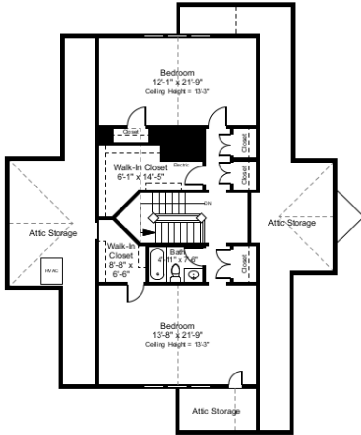
Third Floor Plan Ceiling Height = 7'-10"
